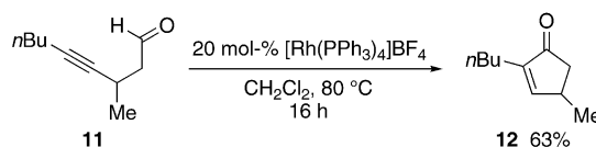
Scheme 12. \text{Rh}^{\text{I}}/\text{PPh}_3 -catalyzed reaction of 4-alkynal.
