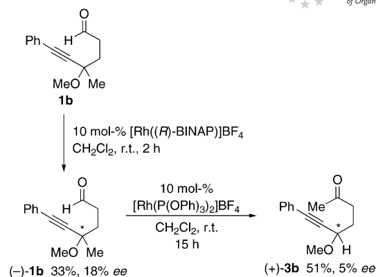
Scheme 4. \text{Rh}^{\text{I}}/\text{P}(\text{OPh})_3 -catalyzed isomerization of enantio-enriched 4-methoxy-5-alkynal (–)- 1b to \gamma -alkynyl ketone (+)- 3b .
