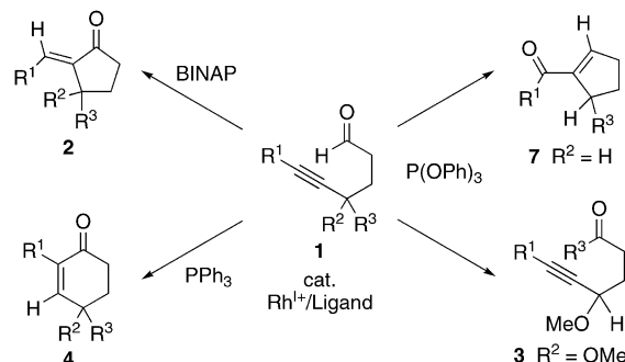
Scheme 15. Effect of ligands and substituents in cationic rhodium(I) complex-catalyzed transformations of 5-alkynals.
