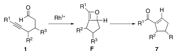
Scheme 9. Possible mechanism for isomerization of 5-alkynals to cyclopent-1-enyl ketones.
