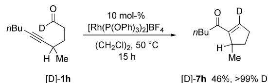
Scheme 10. Deuterium labeling study.
