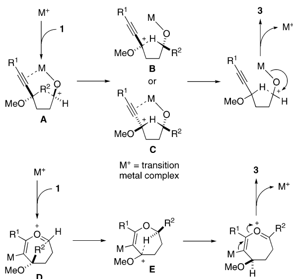
Scheme 7. Possible mechanism for isomerization of 4-methoxy-5-alkynals 1 to \gamma -alkynyl ketones 3 .
