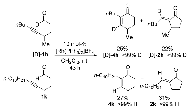
Scheme 14. Crossover deuterium-labeling experiment.
