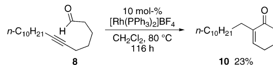
Scheme 11. \text{Rh}^{\text{I}}/\text{PPh}_3 -catalyzed reaction of a 6-alkynal.
