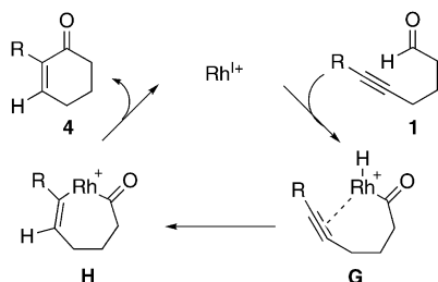
Scheme 13. Possible mechanism for trans hydroacylation of 5-alkynals to give cyclohexenones.
