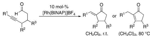
Scheme 2. Rh^{I+}/BINAP -catalyzed reactions of 5-alkynals.
