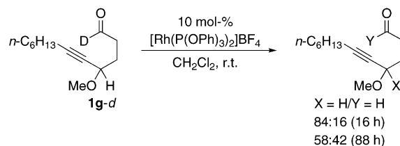
Scheme 6. \text{Rh}^{\text{I}}/\text{P}(\text{OPh})_3 -catalyzed deuterium–hydrogen exchange reaction.
