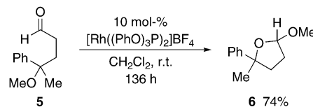
Scheme 5. \text{Rh}^{\text{I}}/\text{P}(\text{OPh})_3 -catalyzed reaction of 4-methoxyaldehyde 5 to give cyclic acetal 6 .
