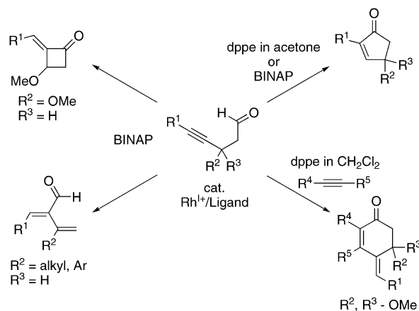
Scheme 1. Effect of ligands and substituents on cationic rhodium(I) complex-catalyzed transformations of 4-alkynals.
