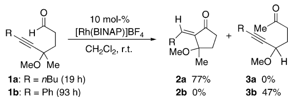
Scheme 3. Rh I +/BINAP-catalyzed reactions of 4-methoxy-5-alkynyls.
