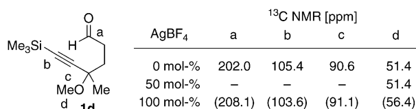
Figure 2. ^{13}\text{C} NMR spectroscopic analysis of 5-alkynal 1d in the presence of \text{AgBF}_4 (numbers in parentheses are the chemical shifts of the isomerization product 3d ).
