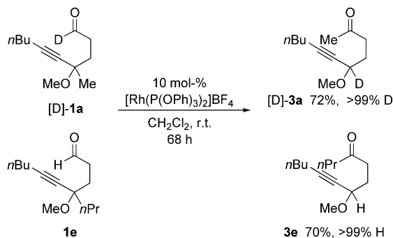
Scheme 8. Crossover deuterium-labeling experiment.
