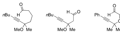
Figure 1. Unsuitable alkynals for \text{Rh}^{\text{I}}/\text{P}(\text{OPh})_3 -catalyzed isomerization to alkynyl ketones.
